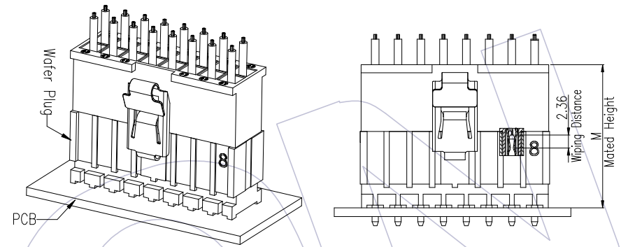
Plug:(S/T DIP TYPE-3)
