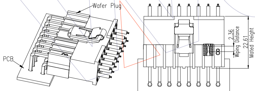
Plug:(R/A DIP TYPE)
