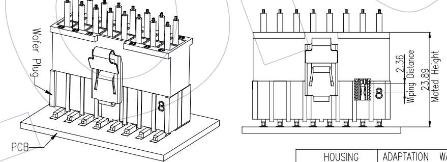
Plug:(S/T SMT TYPE)
